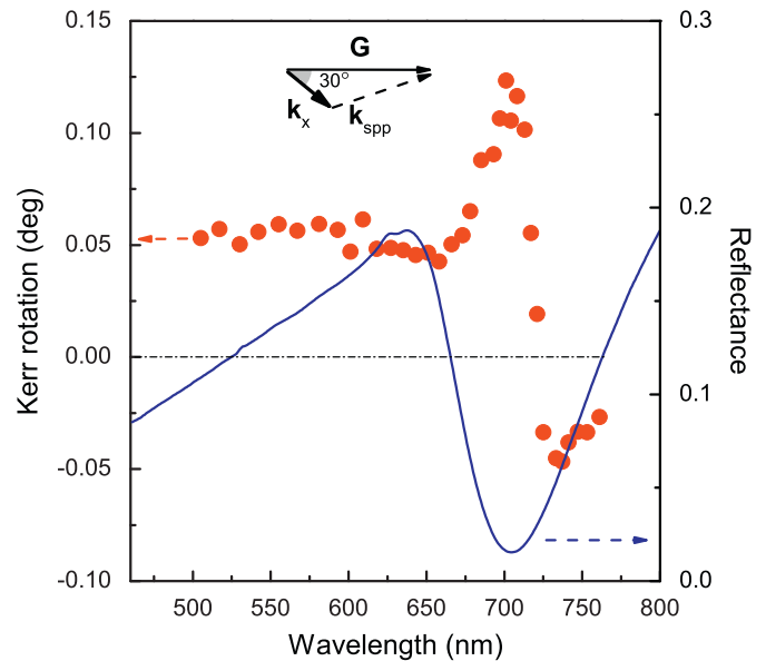
Fig. 3. Spectral dependences of Kerr rotation angle in longitudinal MOKE configuration (circles) and of reflectance (curve) measured in 2D magnetoplasmonic crystal. Angle of incidence is 45°. Inset: schematic of the SPP phase-matching condition.
