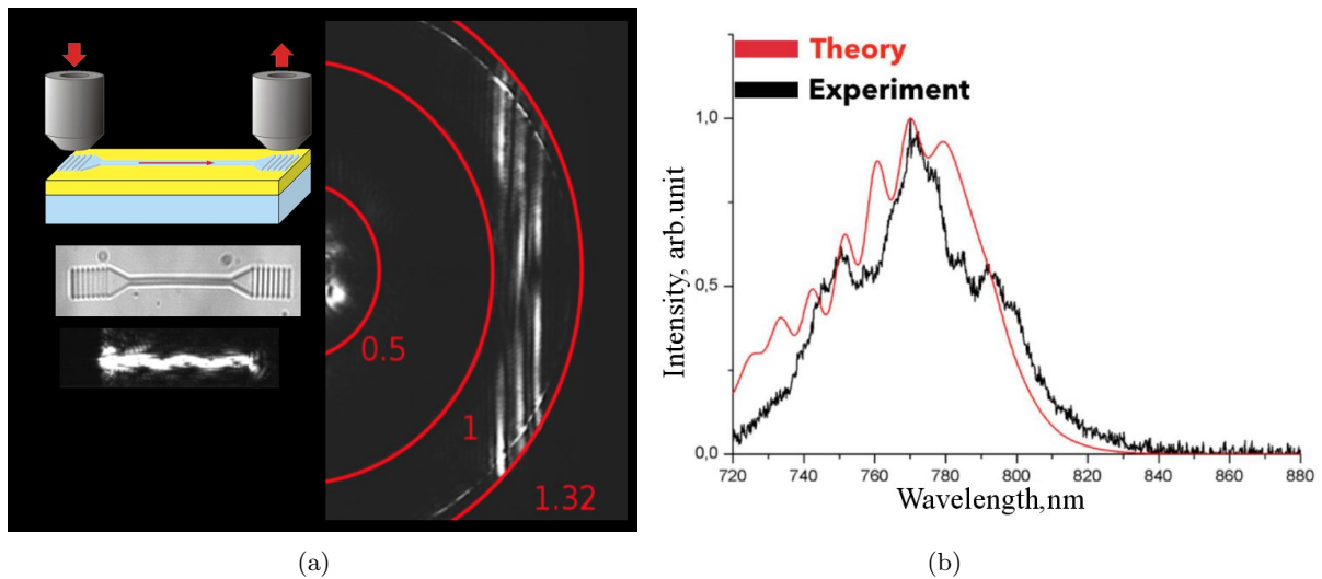
Figure 6: (a) The BFP image and the LR image. (b) Spectrum of light transmitted through the photonic device.
