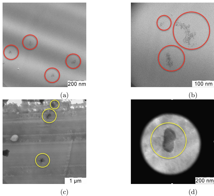
Figure 2: (a,b) TEM images of sample 2 (ORMOCOMP+ QD), QD clusters are marked with red circles, (c,d) TEM images of sample 1 (SU-8 + QD), QD clusters are marked with yellow circles.
