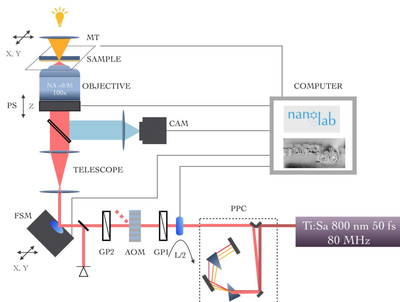
Figure 3: 2PP setup scheme.
