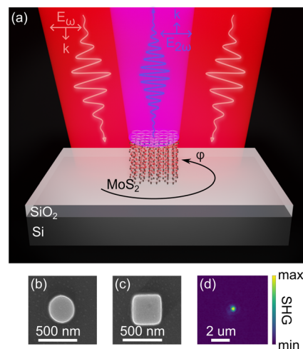
FIGURE 1 | (a) Schematic of the SHG experiment. (b,c) Scanning electron microscope images of cylindrical (b) and cuboid (c) nanoparticles. (d) SH image of a single cubic nanoparticle.
