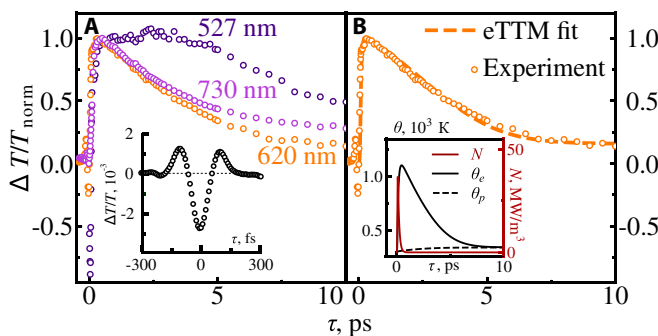
Fig. 4. (A) Experimental temporal dependences of normalized differential transmittance \Delta T / T_{\text{norm}}(\tau) at the 3 wavelengths, corresponding to different resonances: 730 nm (dipole SLR, violet circles), 620 nm (quadrupole SLR, orange circles), and 527 nm (QWG mode, dark purple circles); inset depicts differential transmittance dynamics of the reference flat Bi:YIG layer. (B) Experimental dependence \Delta T / T_{\text{norm}}(\tau) at 620 nm (circles) and its fit by Eq. (3) (dashed line); inset: calculated temporal dependences of nonthermalized electron energy density N(\tau) (red line), temperature of thermalized electrons \theta_e(\tau) (solid black line), and phonon temperature \theta_p(\tau) (dashed line).
