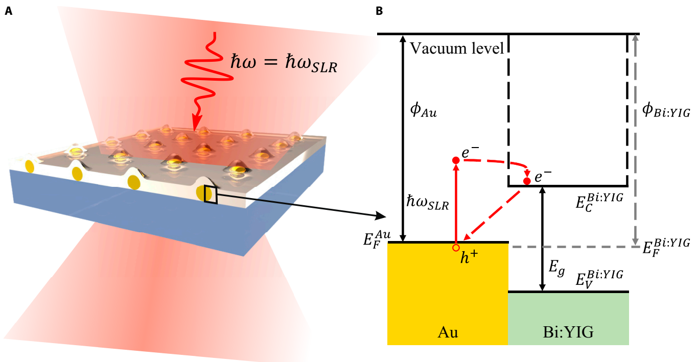
Fig. 1. (A) Scheme of the sample. (B) Schematic energy diagram of the Au/Bi:YIG interface illustrating a possible plasmon-induced hot-carrier injection process.
