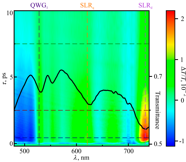
Fig. 2. Black curve: Transmittance spectrum of the Au-Bi:YIG metasurface at an incidence angle of 17°; heat map: differential transmittance dependence on wavelength \lambda and pump-probe time delay \tau , horizontal dashed lines correspond to spectra in Fig. 3, and vertical dashed lines correspond to temporal dependences in Fig. 4.
