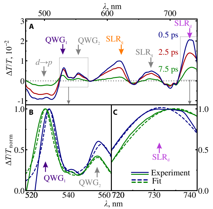
Fig. 3. (A) Experimental differential transmittance spectra \Delta T / T(\lambda) at 3 time delays; arrows indicate spectral positions of the resonances. Normalized to a maximum differential transmittance spectra (solid curves) at the vicinities of the QWG modes (B) and SLR (C) and fit of the spectra (dashed curves) by Eqs. (4) (B) and (5) (C).
