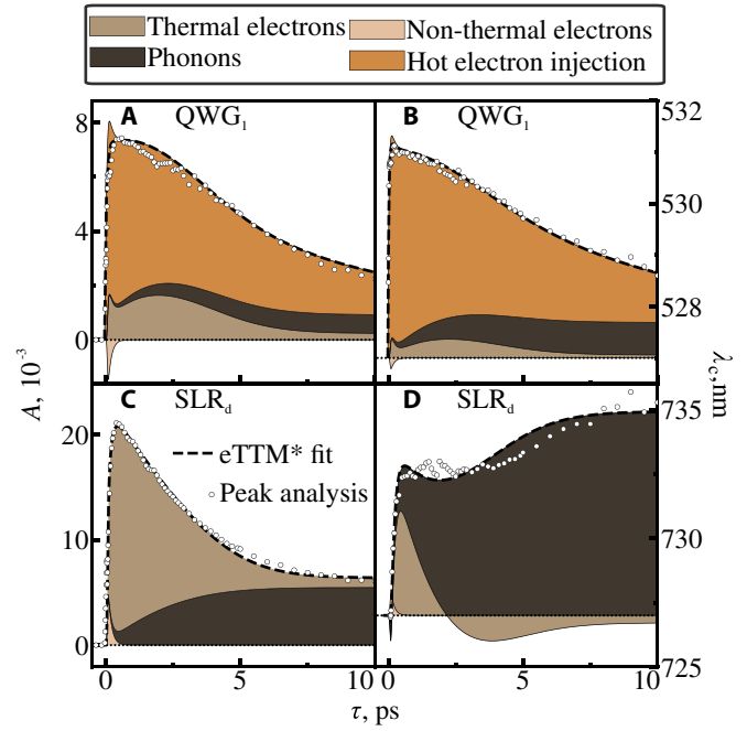
Fig. 5. The temporal dependences of \Delta T / T(\lambda) peak amplitudes A(\tau) (A and C) and their central wavelengths \lambda(\tau) (B and D); circles represent the data obtained from the peak analysis of the experimental spectra by Eqs. (4) and (5); dashed lines correspond to the fits to these data by eTTM* [Eq. (7) for A and B and Eq. (6) for C and D]; (A) and (B) correspond to the analysis of the vicinity the bluish QWG mode, and (C) and (D) correspond to the dipole SLR. The area of the colored regions corresponds to the impacts of the different summands in Eqs. (6) and (7) to the overall dynamics.
